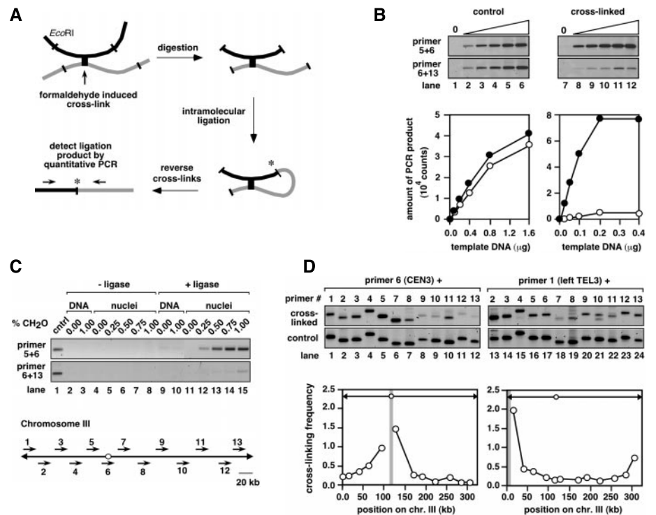
Fig. 1. The Chromosome Conformation Capture (3C) methodology. (A) Schematic representation of the assay: formaldehyde cross-linking, EcoRI digestion, intramolecular ligation, and PCR-mediated detection of ligation products after reversal of the cross-links. The asterisk indicates the newly formed restriction site. (B) Determination of the cross-linking frequency of two loci. The linear range for the quantitative PCR reactions was determined by titrating the cross-linked and control templates, and the products were run on agarose gels. The graphs show the quantitation of PCR product that was obtained with primer pair 5+6 (solid circles) and primer pair 6+13 (open circles) [see (C)]. PCR product formation was linear up to 0.15 μg of cross-linked template and up to 0.4 μg of the control template. In all subsequent experiments, 35 ng of cross-linked template and 150 ng of control template were used. (C) Lower panel: Positions of 13 primers along chromosome III that are used in this study. The open circle indicates the centromere; arrowheads indicate the telomeres. Upper panel: Control experiments. Primer pairs 5+6 and 6+13 were used to detect ligation products on various templates. Similar amounts of ligation products were detected when the control template was used (lane 1). No PCR products were obtained on any of the templates when the ligation step was omitted (lanes 2 to 8). Treating purified genomic DNA with formaldehyde before digestion followed by dilution and ligation did not result in increased ligation product formation (lanes 9 and 10). Using nuclei, no random intermolecular ligation products were detected (lane 11), because no products were detected when the formaldehyde treatment was left out (44). Ligation product formation increased linearly with formaldehyde concentration (lanes 12 to 15). In all other experiments, 1% formaldehyde was used. (D) The method was applied to nuclei isolated from an exponentially growing haploid culture. The cross-linking frequency of the centromere (primer 6, lanes 1 to 12) and the left telomere (primer 1, lanes 13 to 24) with the 12 other sites along chromosome III was determined and plotted. A schematic representation of chromosome III is indicated in which the gray vertical bars represent the position of either the centromere or the left telomere.
