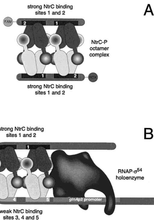
FIGURE 4: Schematic models for the NtrC-P complex with DNA. (A) The octameric complex of NtrC-P with one ES-2 f and one ES-2 r duplex as detected in the FCS/FCCS measurements is shown. Two NtrC dimers drawn in dark or light gray are bound directly to one duplex. Upon phosphorylation of the NtrC receiver domain (represented by a gray-scale gradient), they can associate with each other to form an octamer complex with two separate DNA strands. In the scheme, the two dyes are located on opposite sides of the complex (antiparallel orientation). Since the NtrC binding sites are symmetric, a parallel orientation is equally possible. For a hydrodynamic model of the NtrC-P complex with the ES-2 DNA, see ref 10. According to this model, the separation distance between the two dyes is about 30 nm for an antiparallel orientation and 20 nm for a parallel orientation. (B) Schematic model for a possible conformation of the looped intermediate formed between the octamer complex of NtrC-P and RNAP-σ 54 at the glnAp2 promoter. Two NtrC dimers are bound to strong sites 1 and 2 (template positions -148 to -132 and -116 to -100). Two additional NtrC dimers (light gray) can associate with the two DNA-bound dimers to form a NtrC octamer complex and could interact with the weak binding sites close to the promoter.
